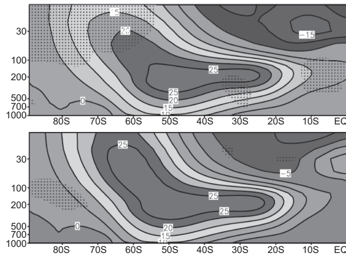
Fig. 9. Latitude versus pressure profile of composite of zonal mean wind ( \text{ms}^{-1} - filtered): (top) easterly QBO, and (bottom) westerly QBO. Areas with 90% significance are dotted (t-student test).
