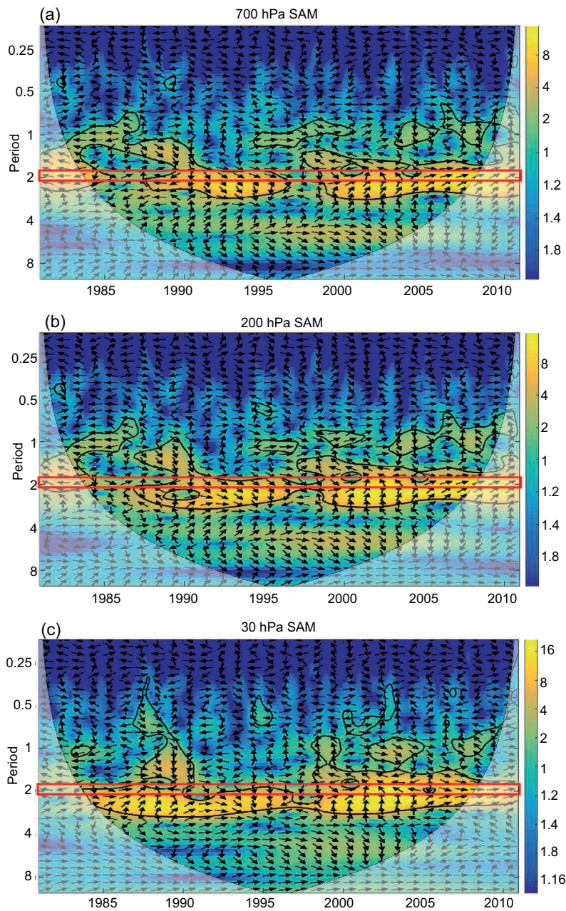
Fig. 2. Cross-wavelet transform (XWT) of the QBO and SAM index time series. The thick black contour designates the 5% significance level. The relative phase relationship is shown as arrows, with in-phase pointing right, anti-phase pointing left, the QBO leading SAM by 90^\circ ( 270^\circ ) pointing straight down (up). The red rectangle displays the 2-year band.
